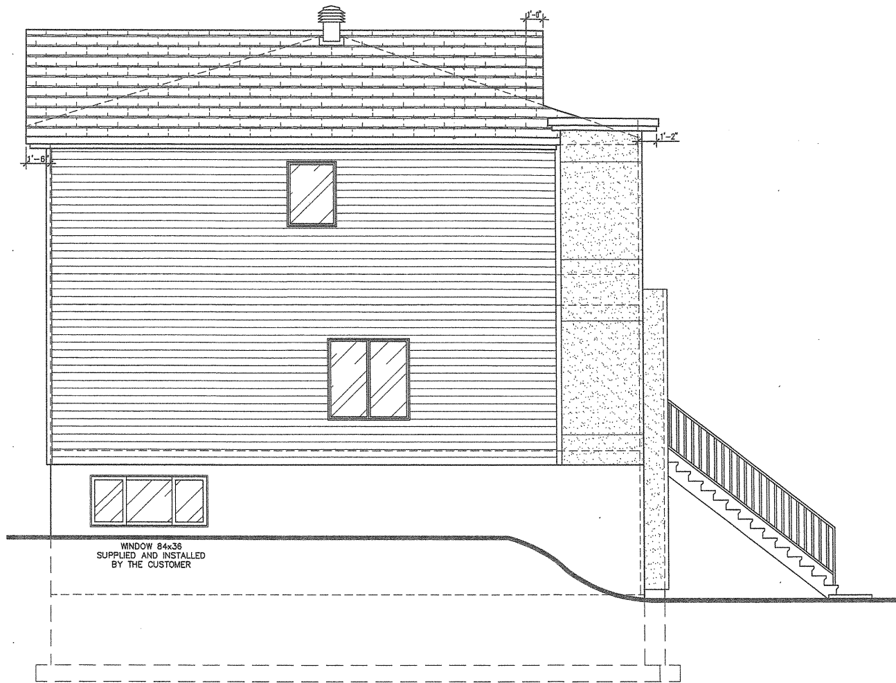
LEFT ELEVATION
